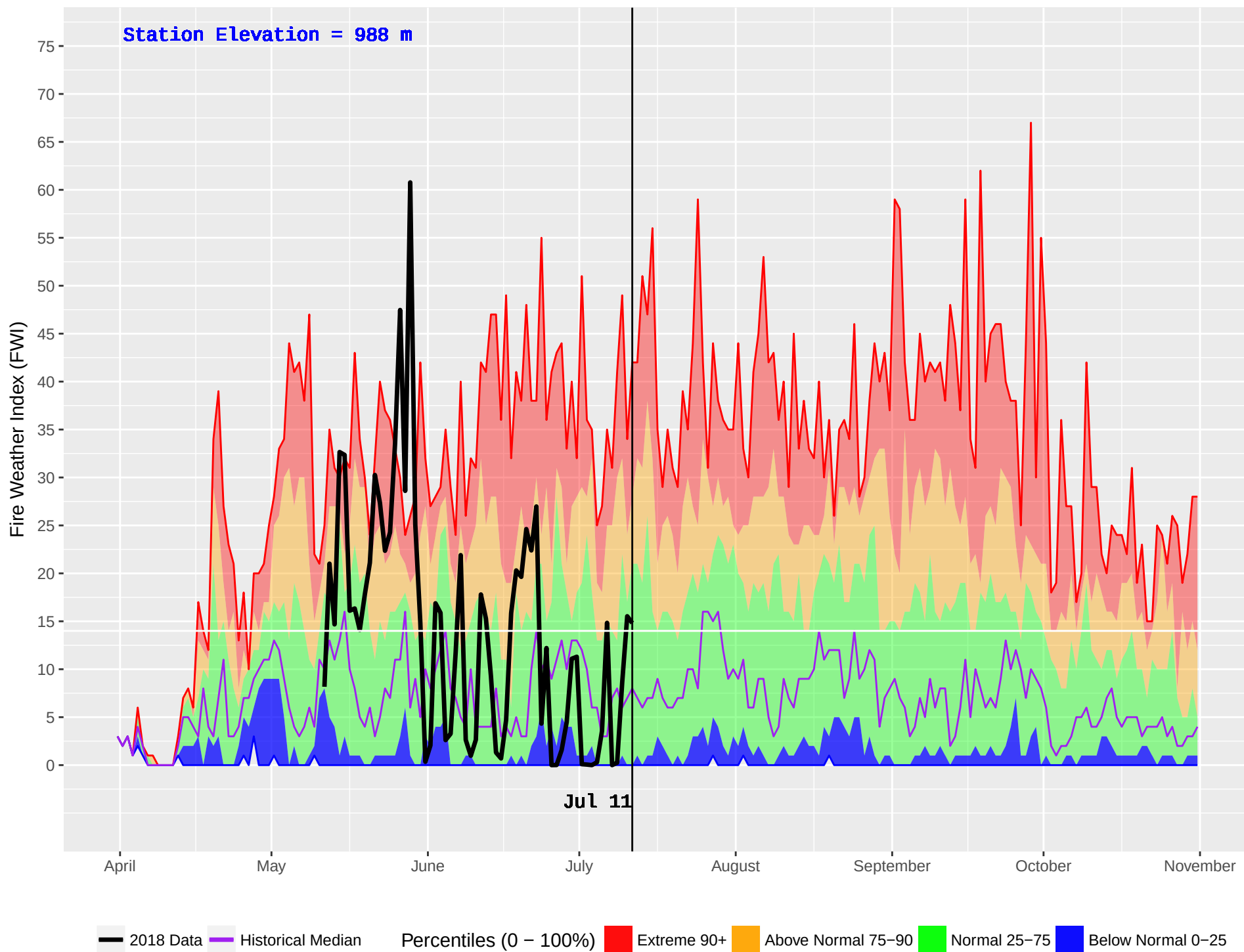
NOEL (437) : Historical (1993–2016) and Current (2018) Noon Fire Weather Index (FWI)
