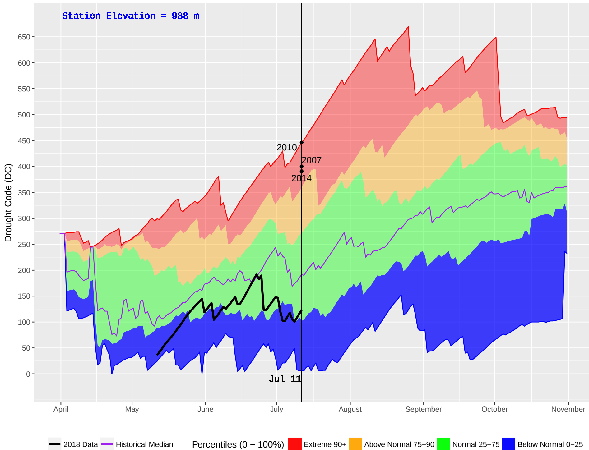
NOEL (437) : Historical (1993–2016) and Current (2018) Noon Drought Code (DC)
