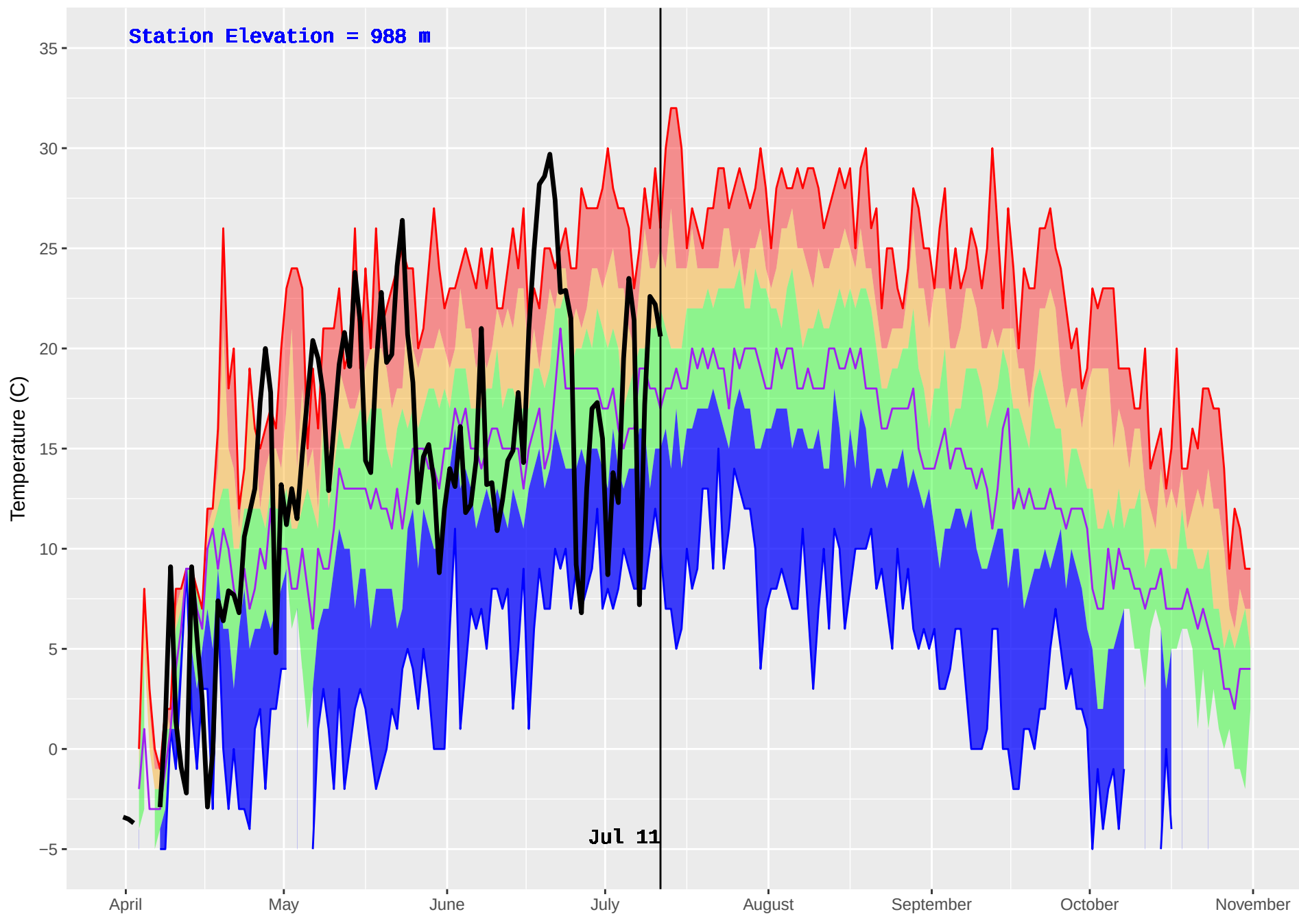
NOEL (437) : Historical (1993–2016) and Current (2018) Noon Temperature
